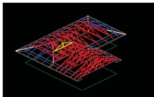
Top chord load test
