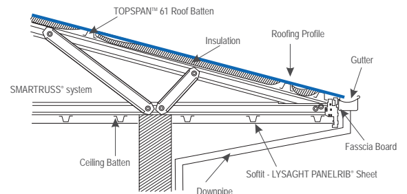
Cross section of SMARTRUSS® roofing system
